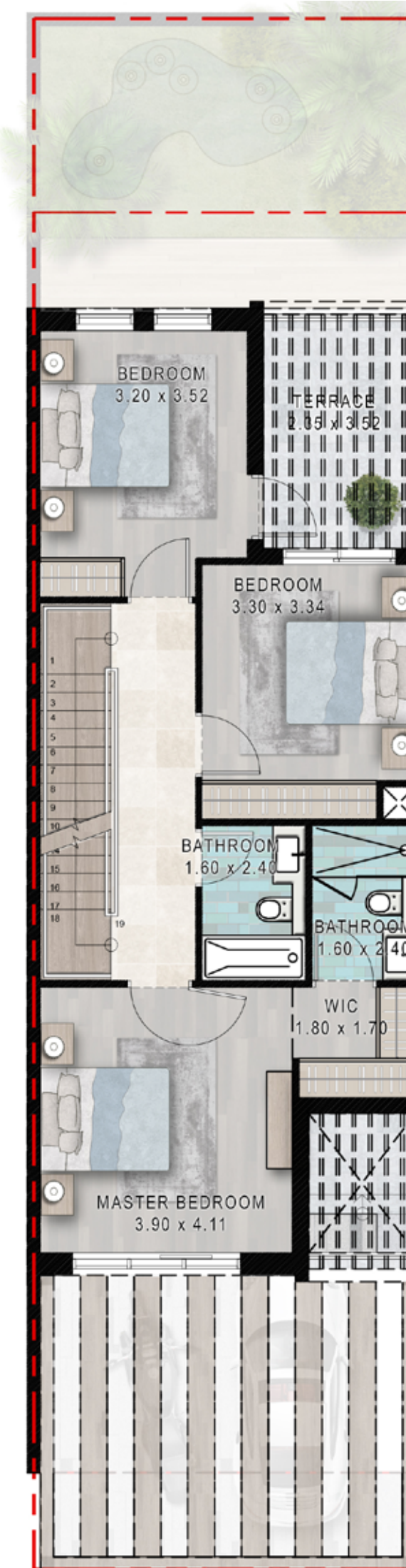
FIRST FLOOR
